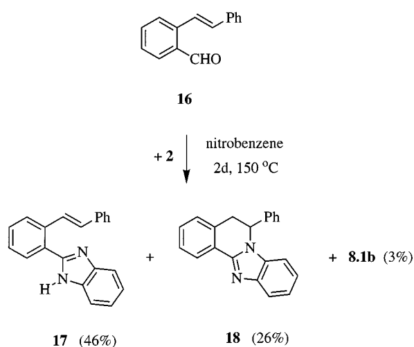
Scheme 5. Products of the oxidative cyclization of functionalized stilbene 16 with ortho -phenylenediamine ( 2 )
